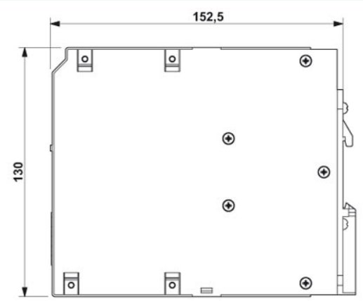
Dimensioned drawing
